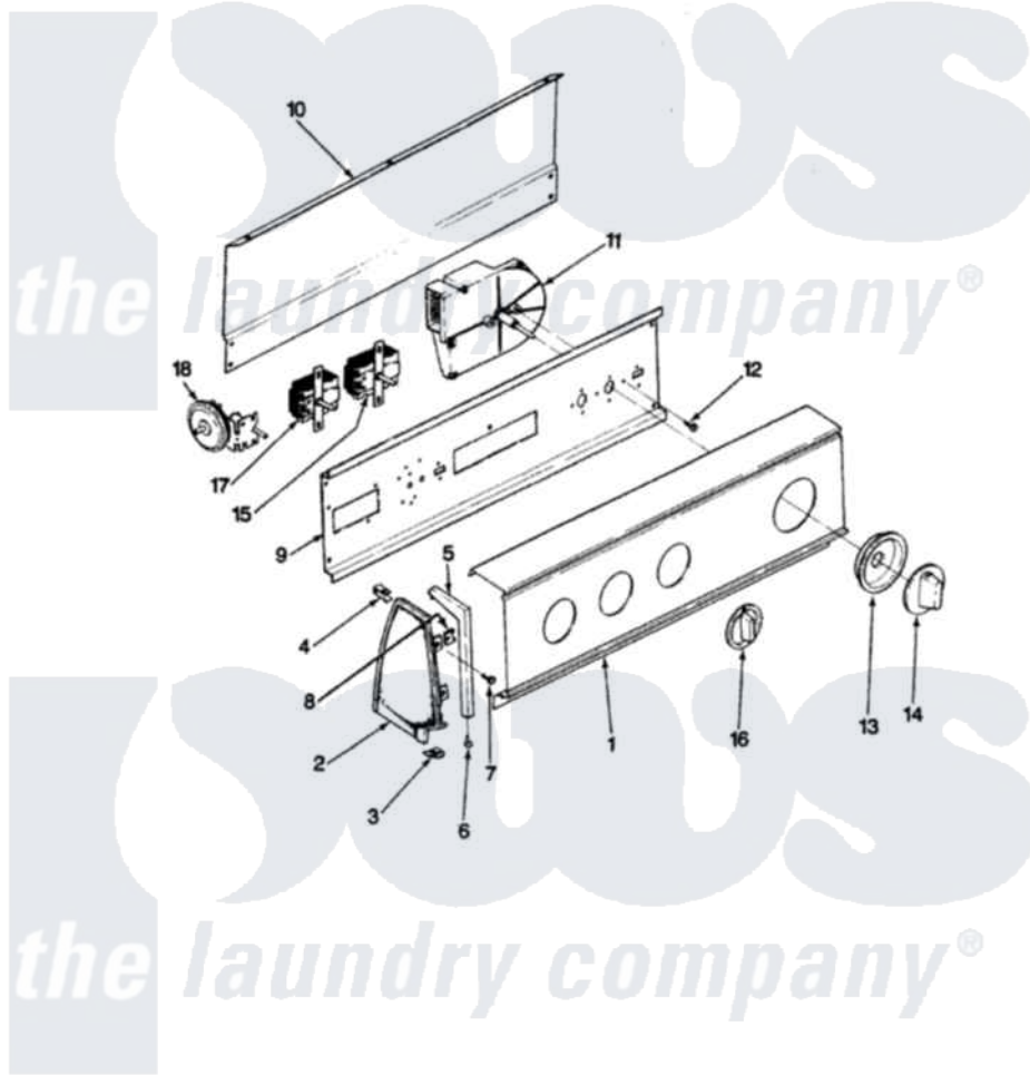
Admiral Residential Admiral AW25K3AS Washer Parts Parts Diagram 03 - CONTROL PANEL Click on the part number to view part
