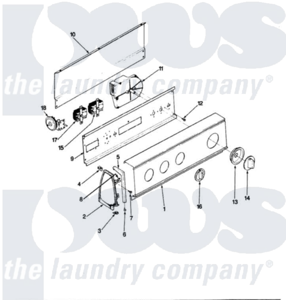
Admiral Residential Admiral AW26L3AK Washer Parts Parts Diagram 02 - CONTROL PANEL (REV. A-D) Click on the part number to view part
