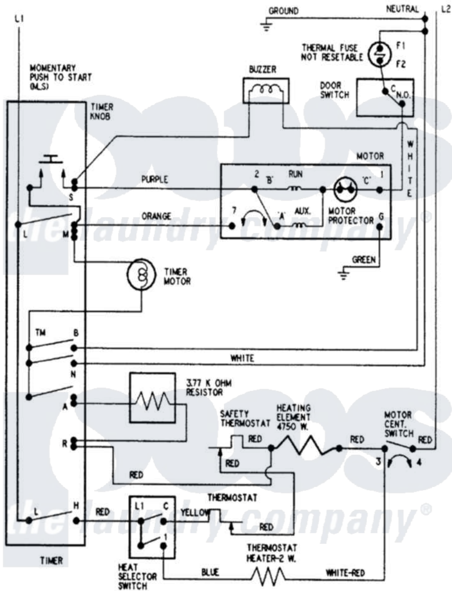
Admiral Residential Admiral AYE2250AYW Dryer Parts Parts Diagram 06 - WIRING INFORMATION Click on the part number to view part
