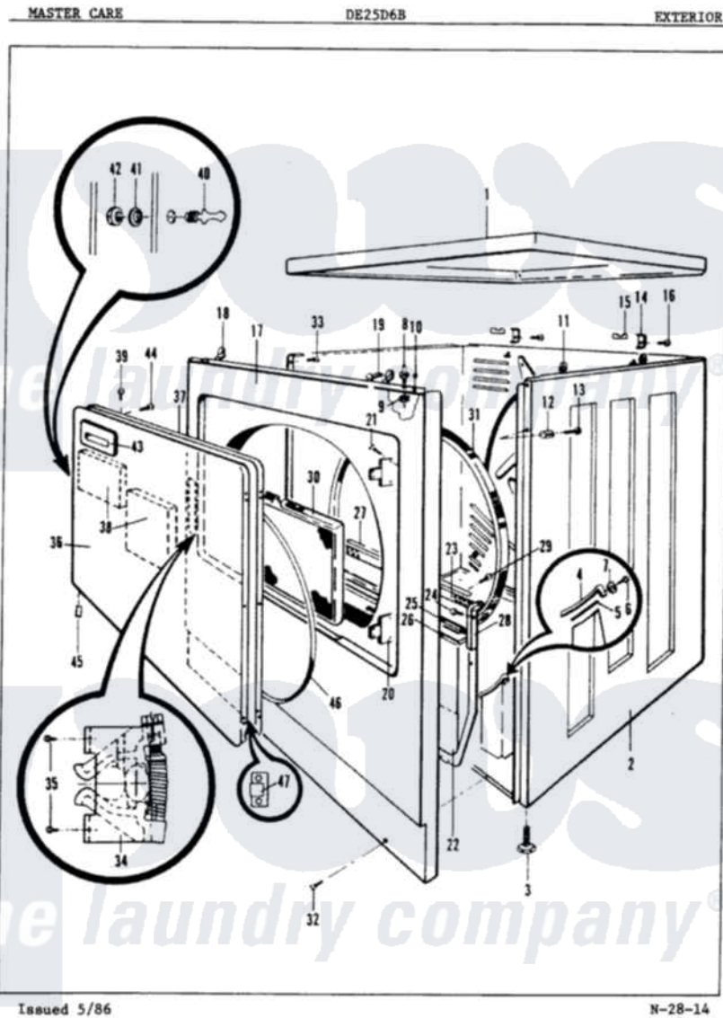
Admiral Residential Admiral DE25D6B Dryer Parts Parts Diagram 05 - EXTERIOR Click on the part number to view part
