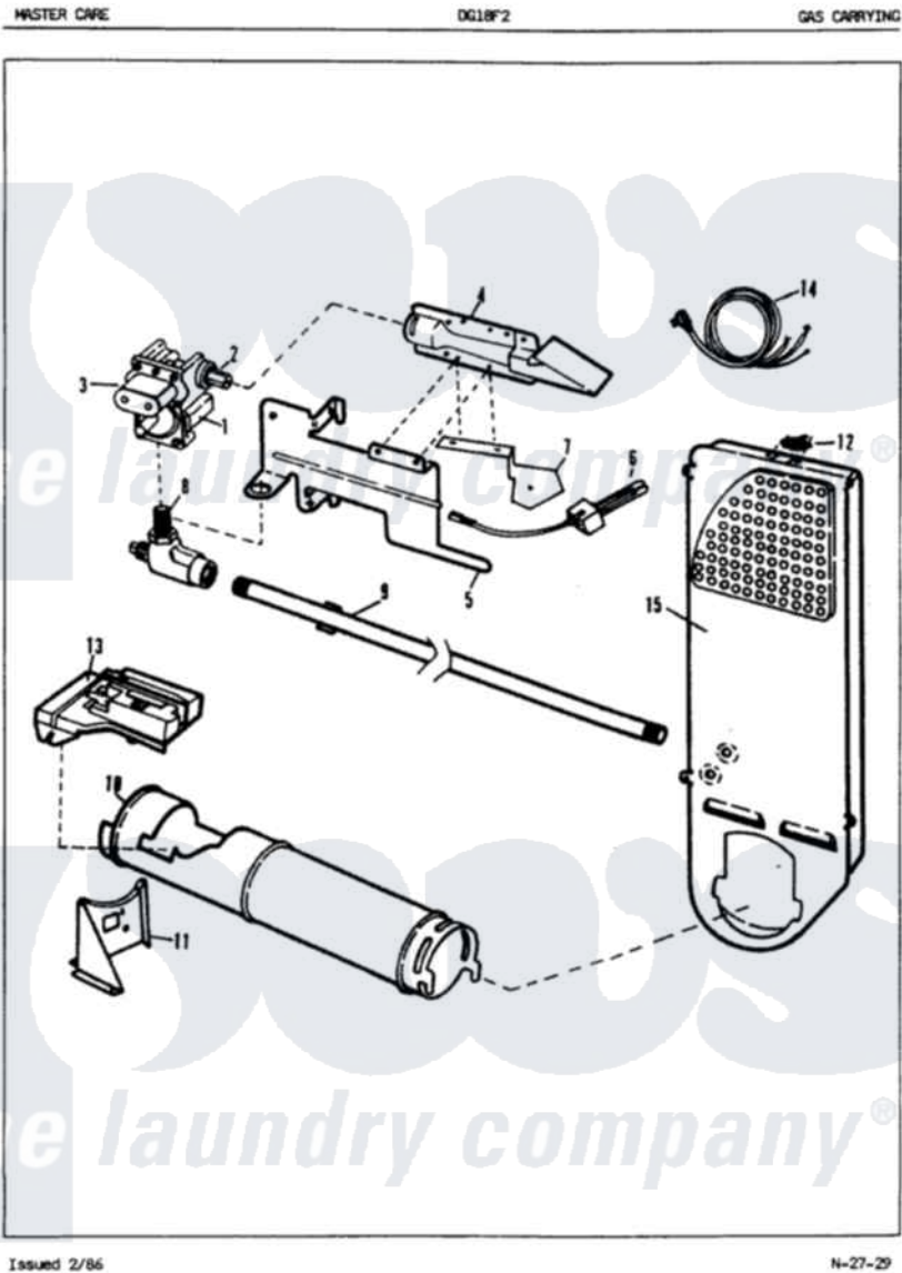
Admiral Residential Admiral DG18F2WN Dryer Parts Parts Diagram 04 - GAS CARRYING Click on the part number to view part
