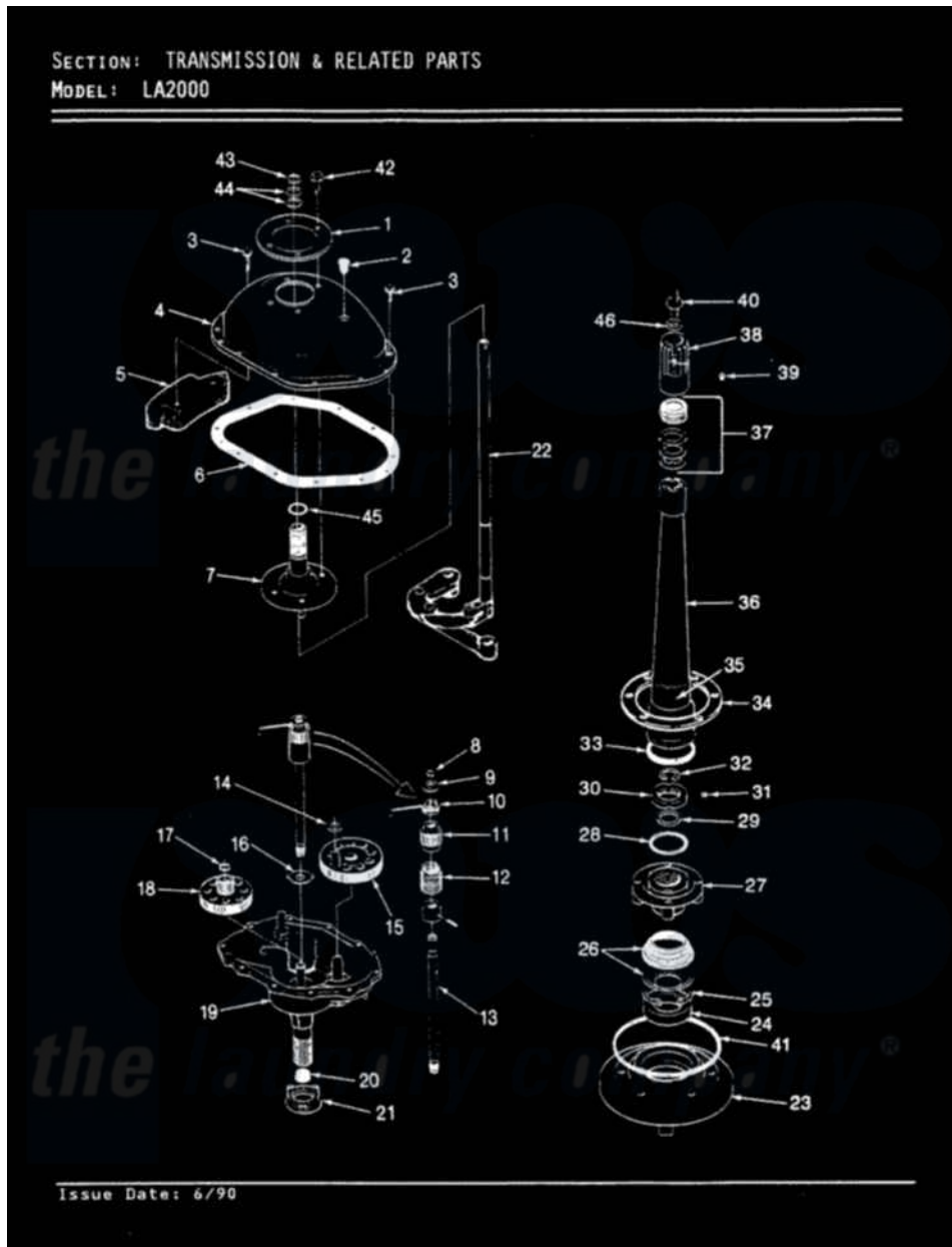
Admiral Residential Admiral LA2000A Dryer Parts Parts Diagram 06 - TRANSMISSION (REV. E-F) Click on the part number to view part
