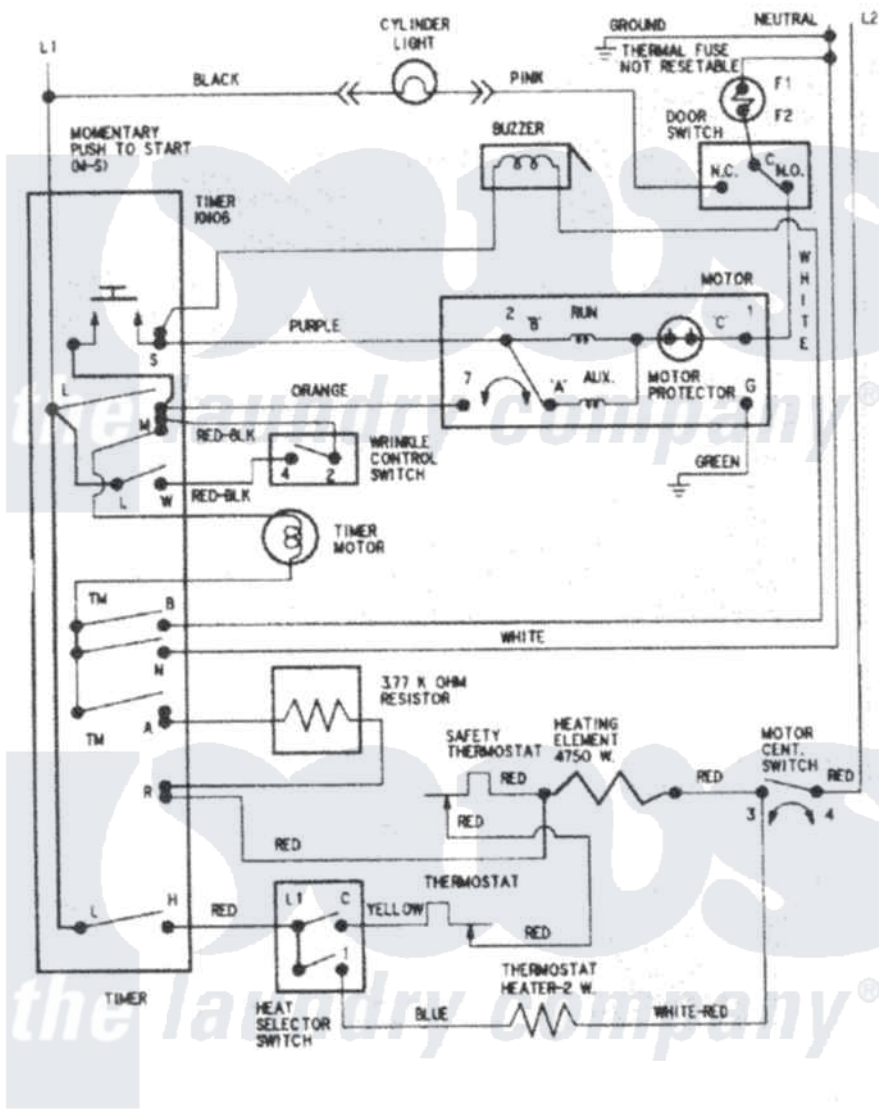
Admiral Residential Admiral LNC7766B71 Dryer Parts Parts Diagram 09 - WIRING INFORMATION Click on the part number to view part
