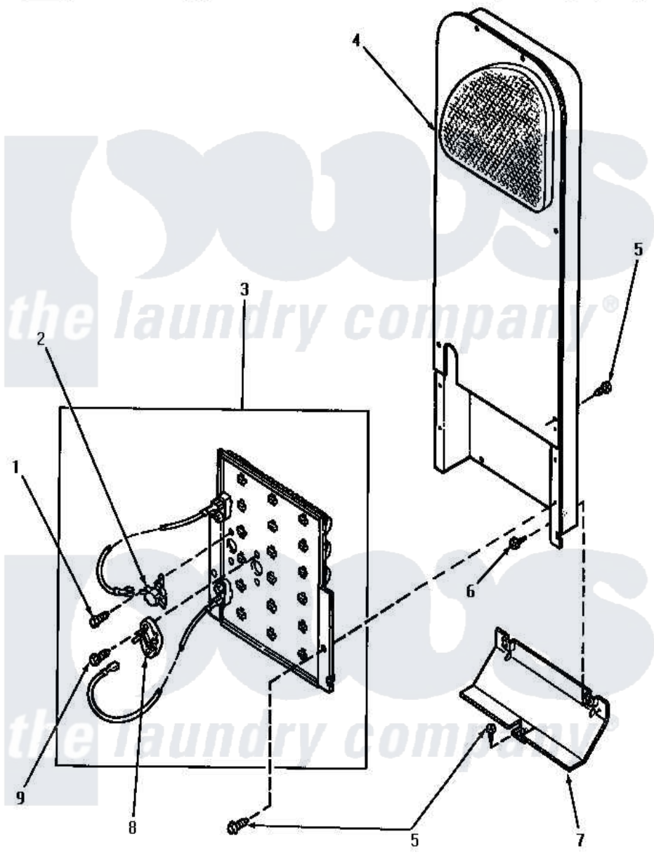
Amana Residential Amana AEM353 Dryer Parts Parts Diagram 06 - HEATER BOX Click on the part number to view part
