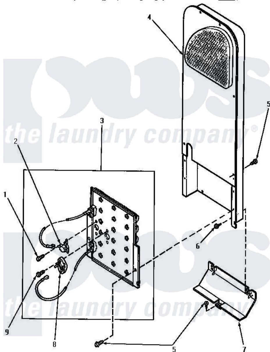
Amana Residential Amana AEM433 Dryer Parts Parts Diagram 06 - HEATER BOX Click on the part number to view part
