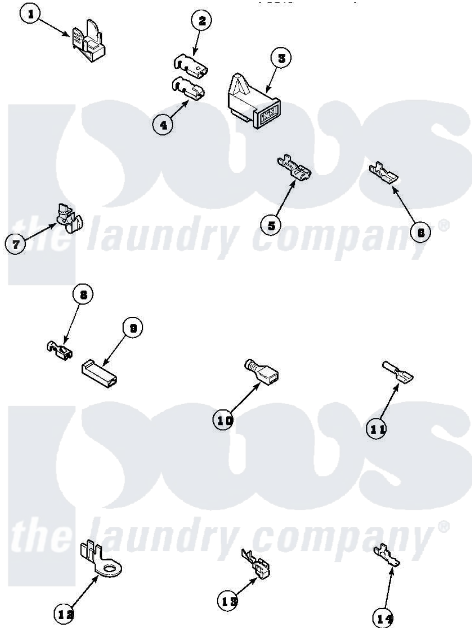
Amana Residential Amana AEM497W2 (BOM: PAEM497W2) Dryer Parts Parts Diagram 18 - TERMINALS Click on the part number to view part
