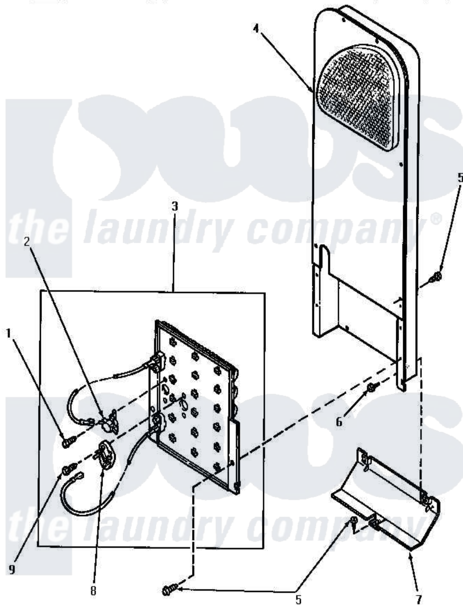
Amana Residential Amana AEM653 Dryer Parts Parts Diagram 06 - HEATER BOX Click on the part number to view part
