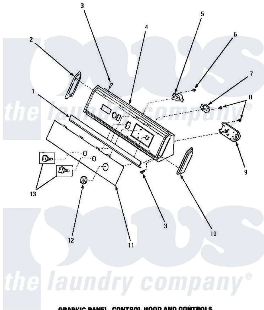
GRAPHIC PANEL, CONTROL HOOD AND CONTROLS (Models AEM677*2, ARM678*2, AEM697*2 and AGM699*2) *Is the color designator, "L" indicates ALMOND color and "W" indicates WHITE color.
