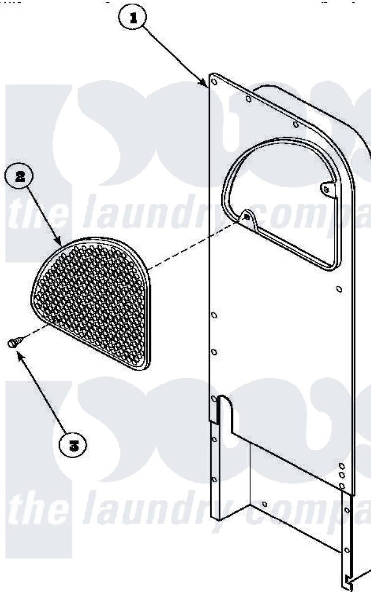
Amana Residential Amana AEM697L2 (BOM: PAEM697L2) Dryer Parts Parts Diagram 10 - HEATER BOX ASSY REPLACEMENT
