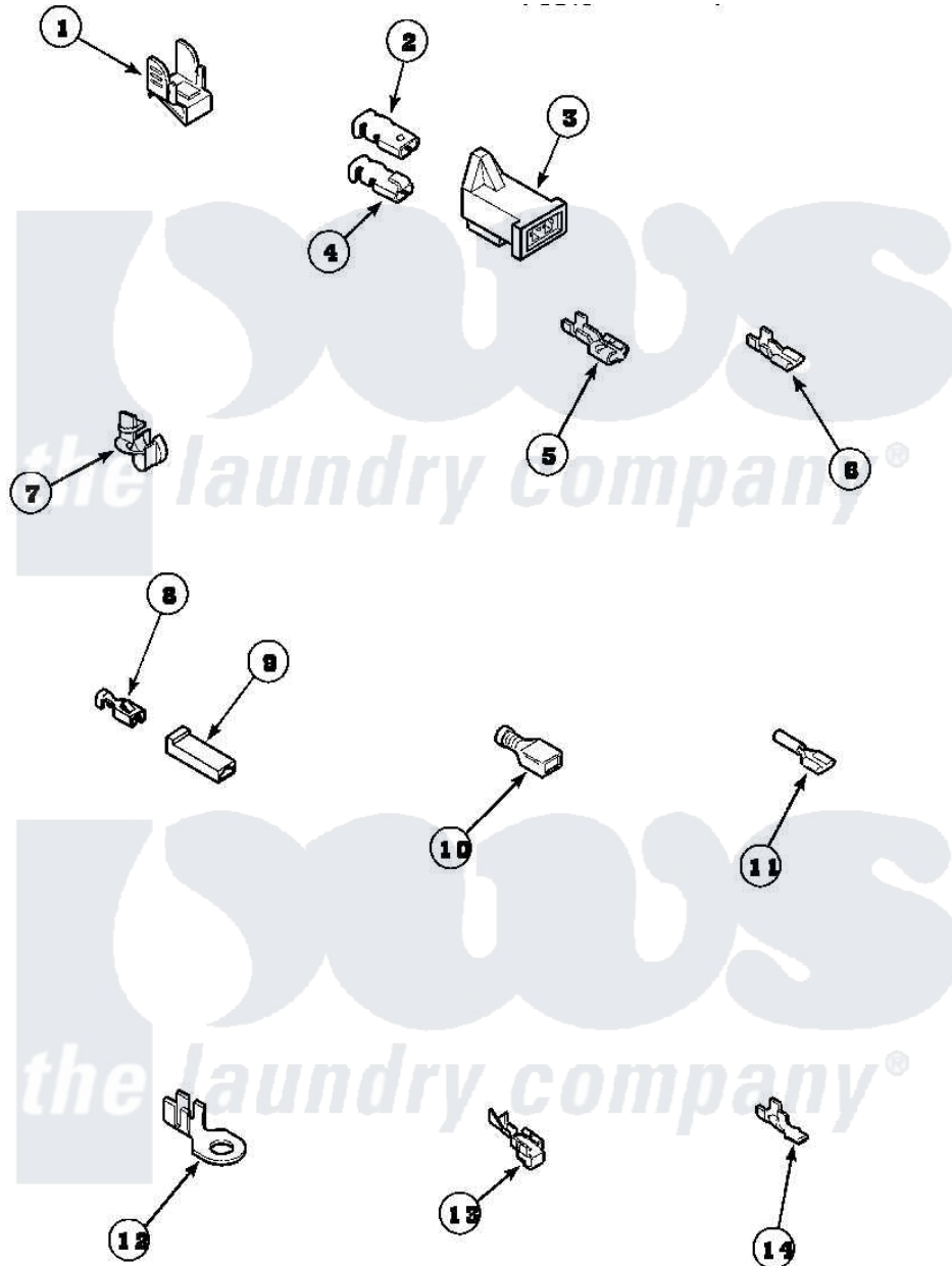
Amana Residential Amana AGM409W2 (BOM: PAGM409W2) Dryer Parts Parts Diagram 18 - TERMINALS Click on the part number to view part
