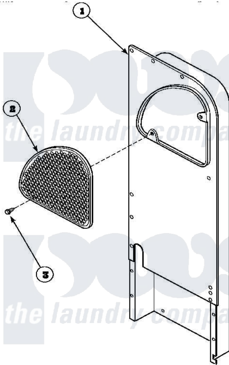
Amana Residential Amana AGM499W2 (BOM: PAGM499W2) Dryer Parts Parts Diagram 10 - HEATER BOX ASSY REPLACEMENT
