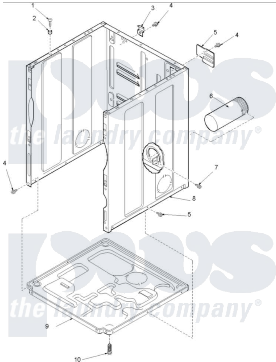
Amana Residential Amana ALE665SAW (BOM: PALE665SAW) Dryer Parts Parts Diagram 01 - CABINET AND BASE
