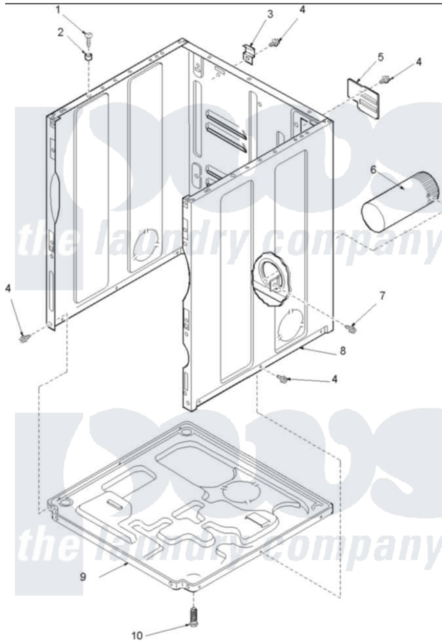
Amana Residential Amana ALE866SAW (BOM: PALE866SAW) Dryer Parts Parts Diagram 01 - CABINET AND BASE Click on the part number to view part
