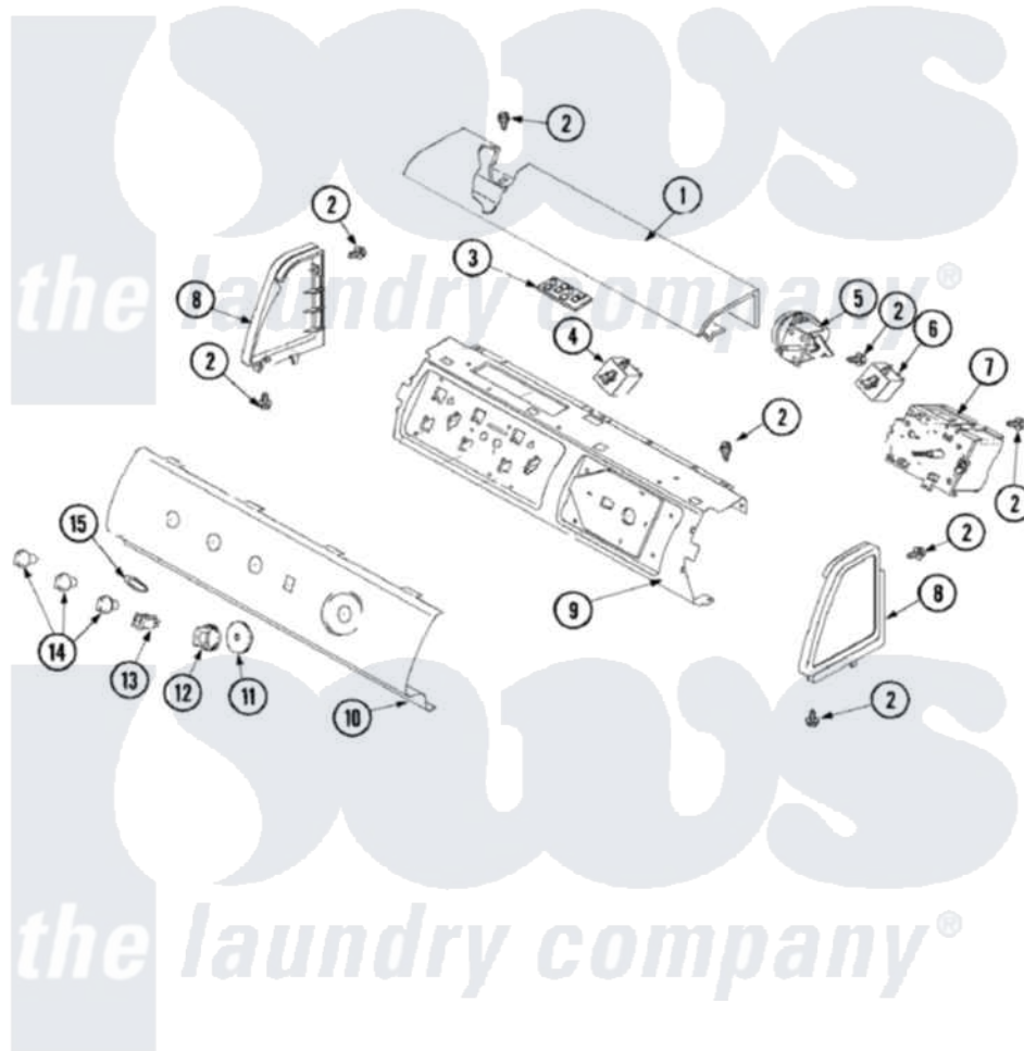
Amana Residential Amana ALW895SAW Washer Parts Parts Diagram 02 - CONTROL PANEL Click on the part number to view part
