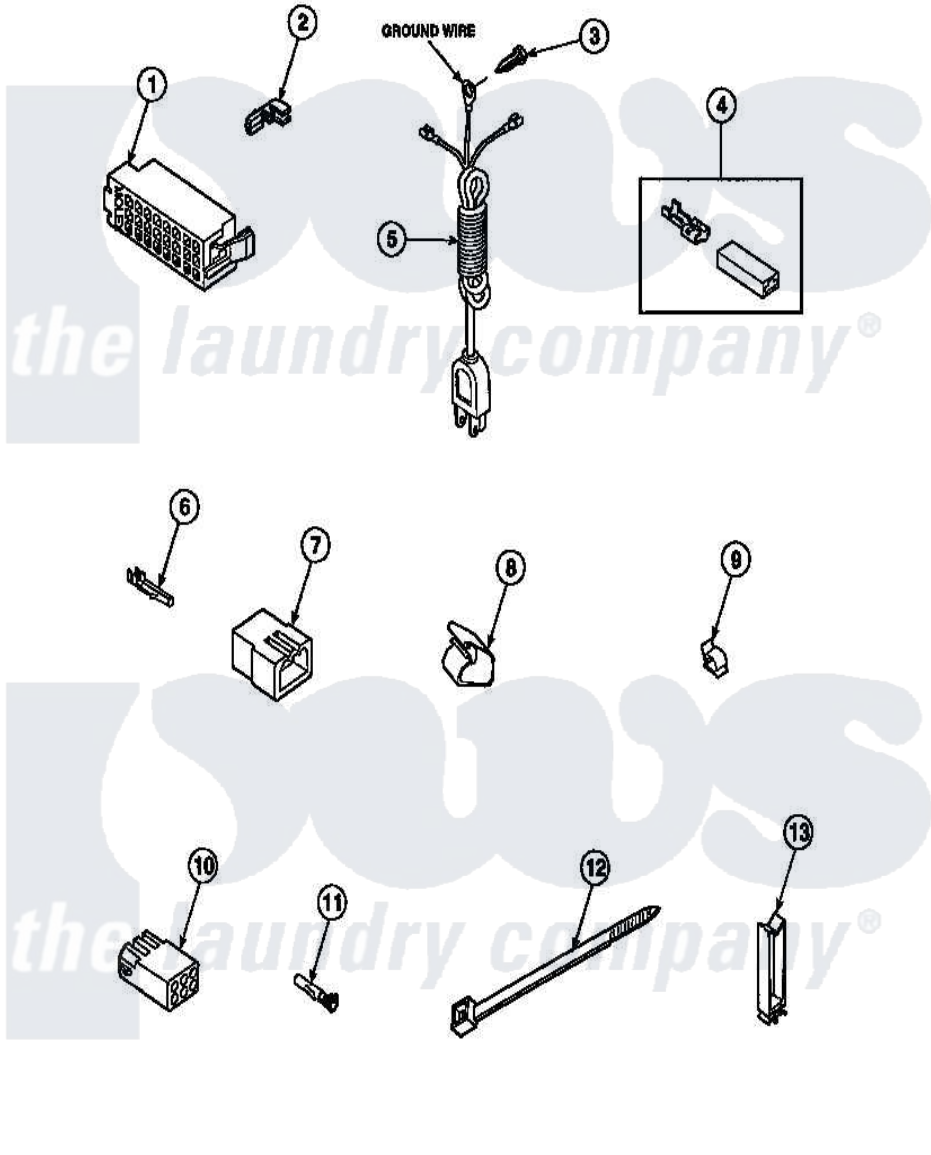
Amana Residential Amana AWM270W2 (BOM: PAWM270W2) Washer Parts Parts Diagram 18 - POWER CORD AND TERMINALS
