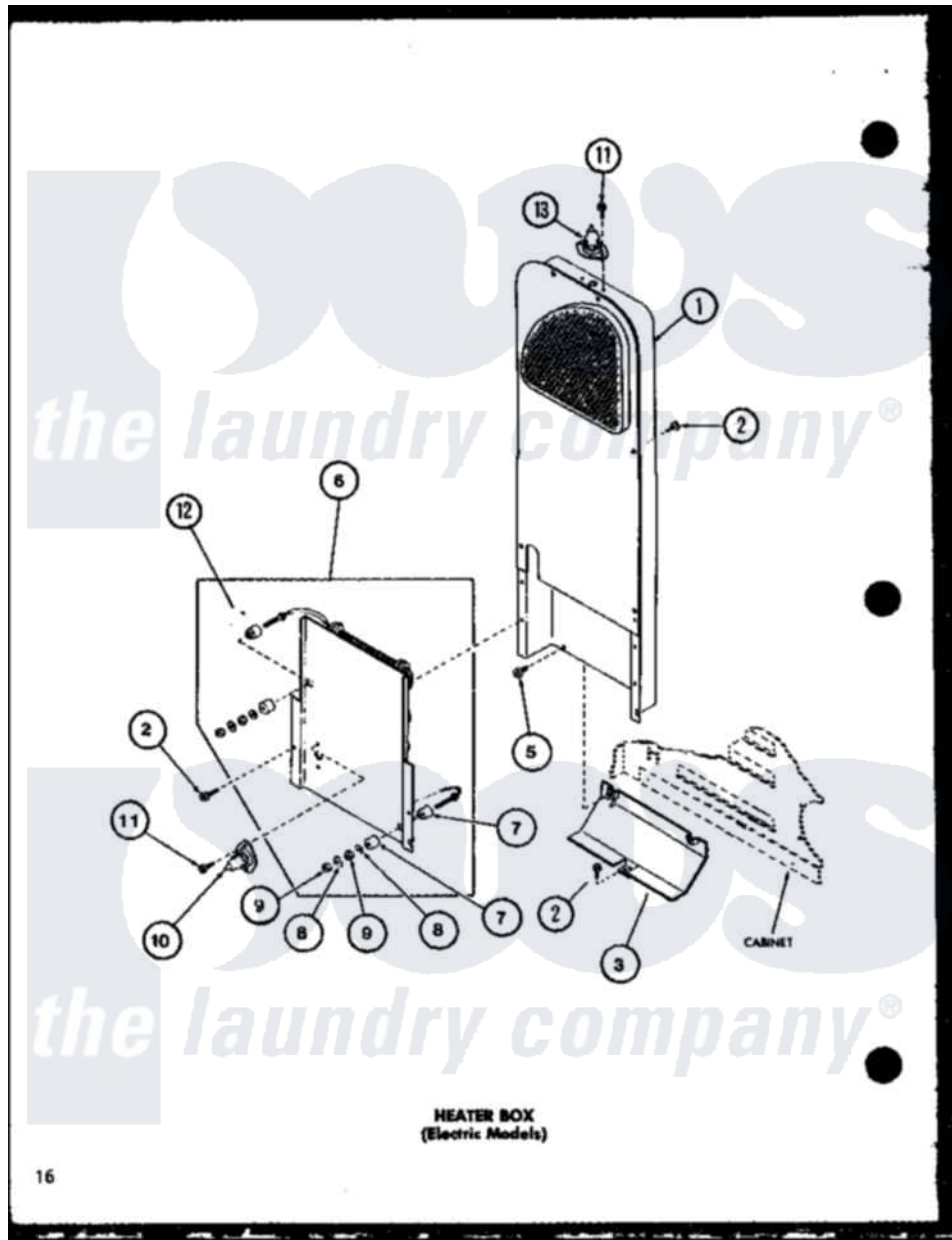
Amana Residential Amana CE2402 (BOM: P7762235W) Dryer Parts Parts Diagram 03 - HEATER BOX (ELECTRIC MODELS)
