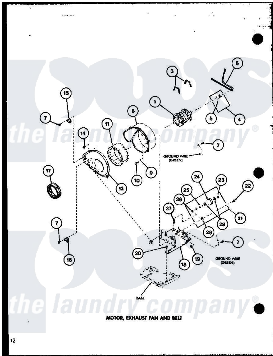
Amana Residential Amana CE2402 (BOM: P7762235W) Dryer Parts Parts Diagram 05 - MOTOR Click on the part number to view part
