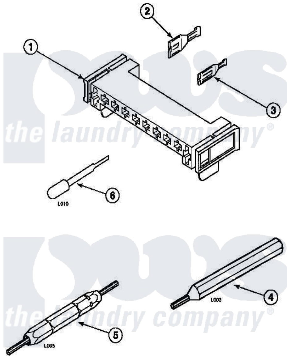
Amana Residential Amana CE8317W2 (BOM: PCE8317W2) Dryer Parts Diagram 16 - Page 21 Click on the part number to view part
