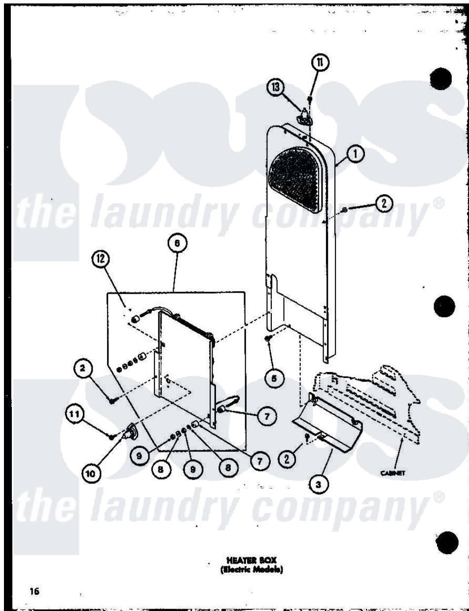
Amana Residential Amana CE9002 (BOM: P7804829W) Dryer Parts Parts Diagram 03 - HEATER BOX (ELECTRIC MODELS)
