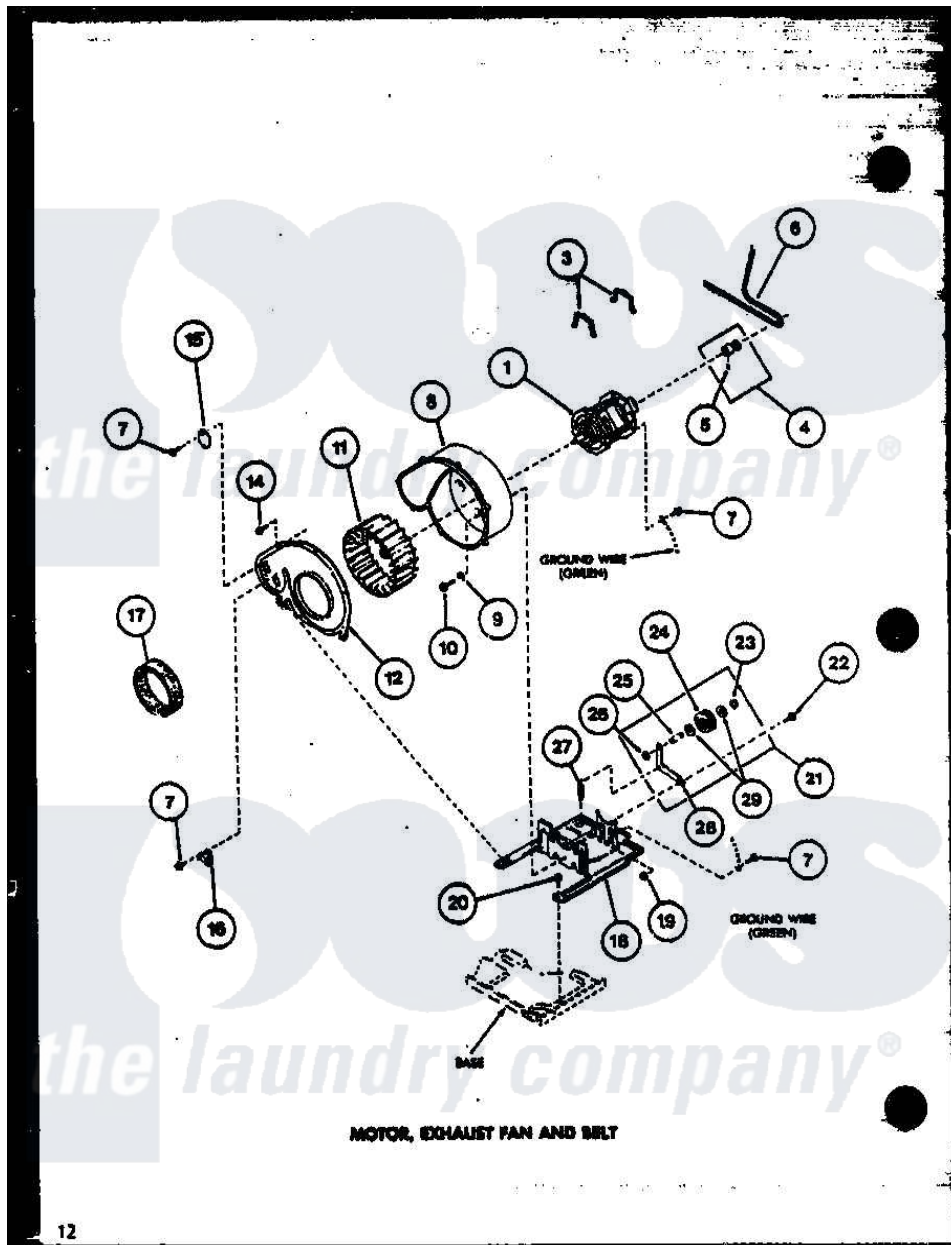
Amana Residential Amana CE9002 (BOM: P7804829W) Dryer Parts Parts Diagram 05 - MOTOR
