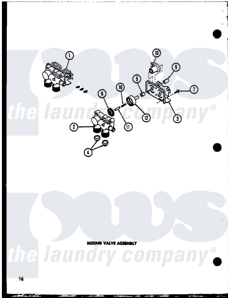
Amana Residential Amana CW2303G (BOM: P1122908W G) Washer Parts Parts Diagram 03 - MIXING VALVE ASSY
