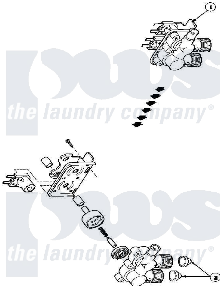
Amana Residential Amana CW8202W2 (BOM: PCW8202W2 B) Washer Parts Parts Diagram 18 - MIXING VALVE
