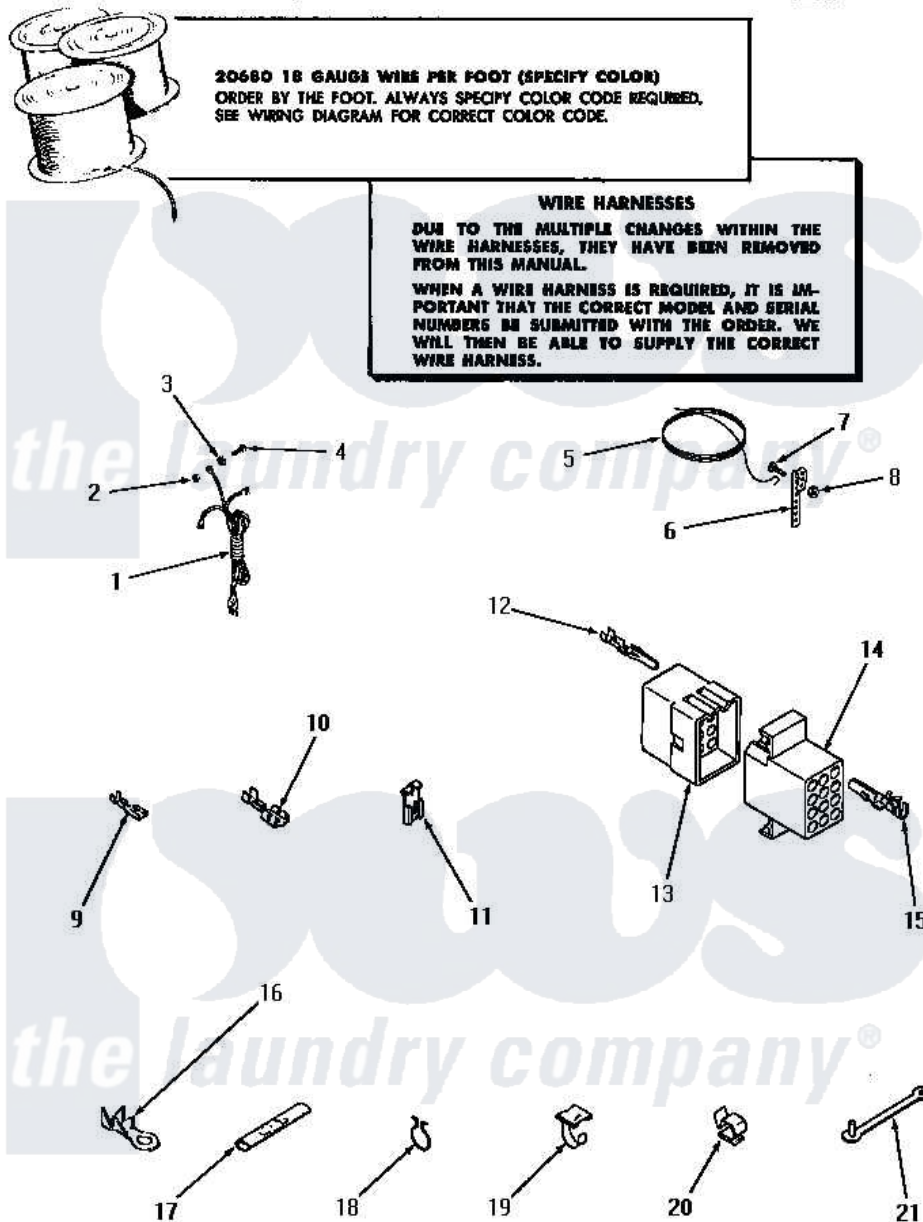
Amana Residential Amana DA1040 Washer Parts Parts Diagram 16 - POWER CORD, WIRE AND TERMINALS Click on the part number to view part
