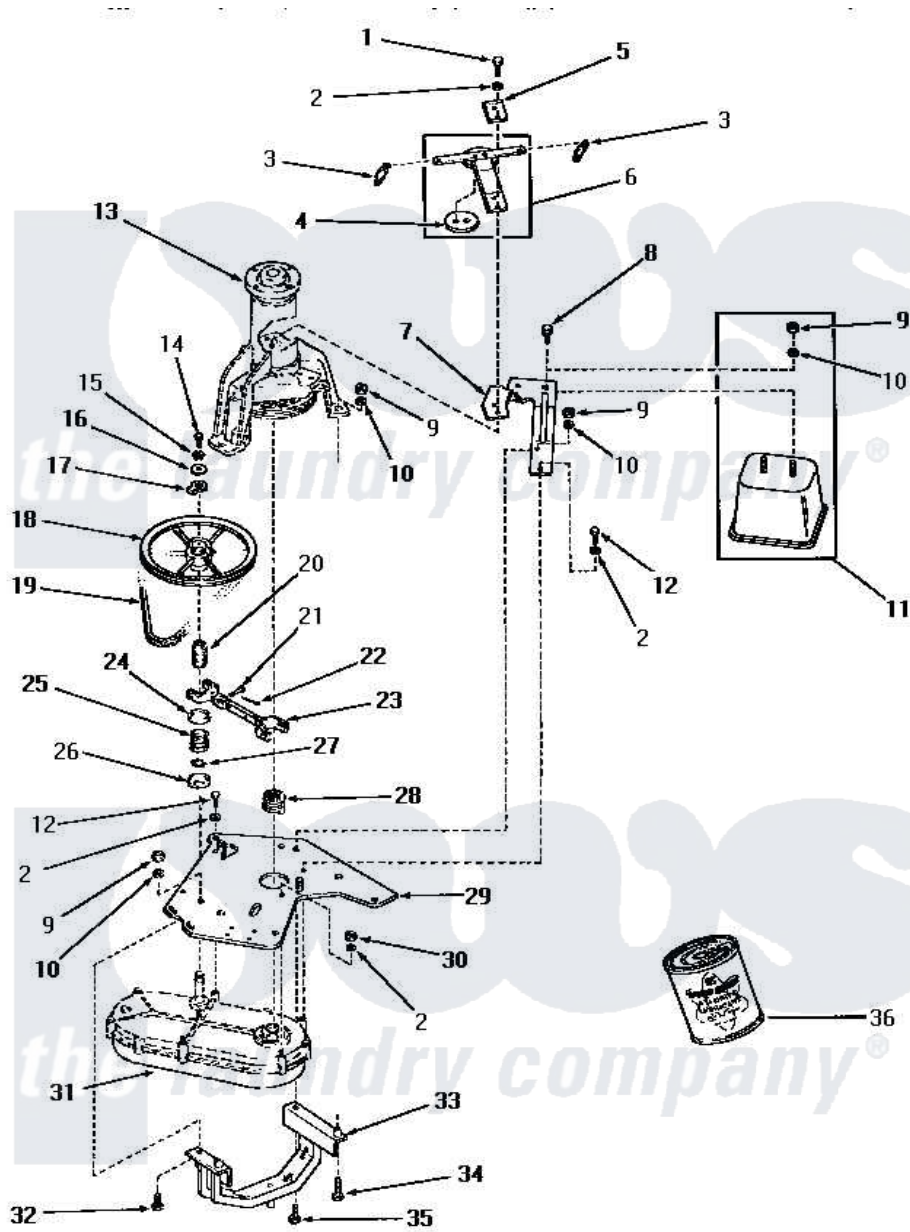
Amana Residential Amana DA6111 Washer Parts Parts Diagram 13 - COUNTERBALANCE, WEIGHT, BRKT & MTG PLATE
