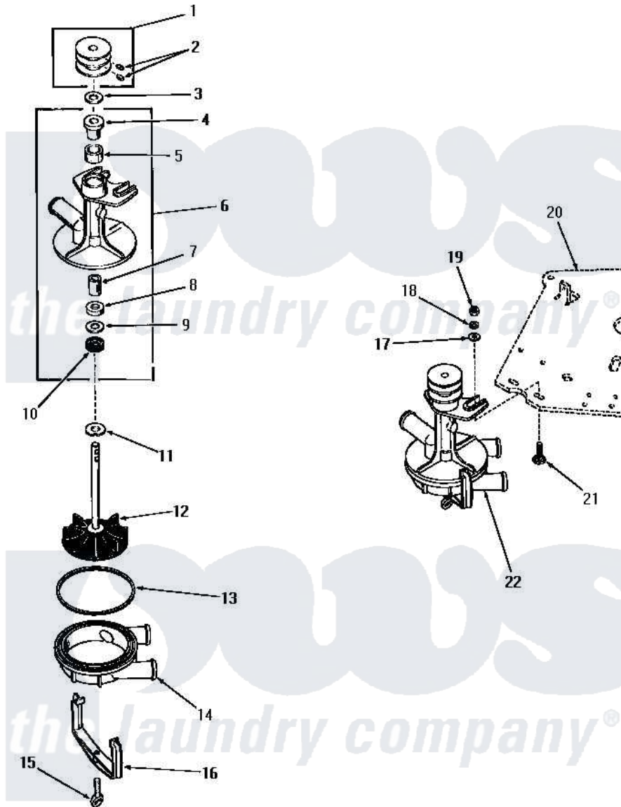
23907 AND 24304 PUMP ASSEMBLIES
