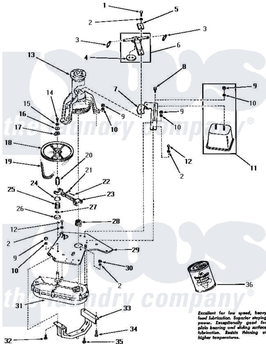
Amana Residential Amana DA6200 Washer Parts Parts Diagram 11 - COUNTERBALANCE WEIGHT, BRKT & MTG PLATE
