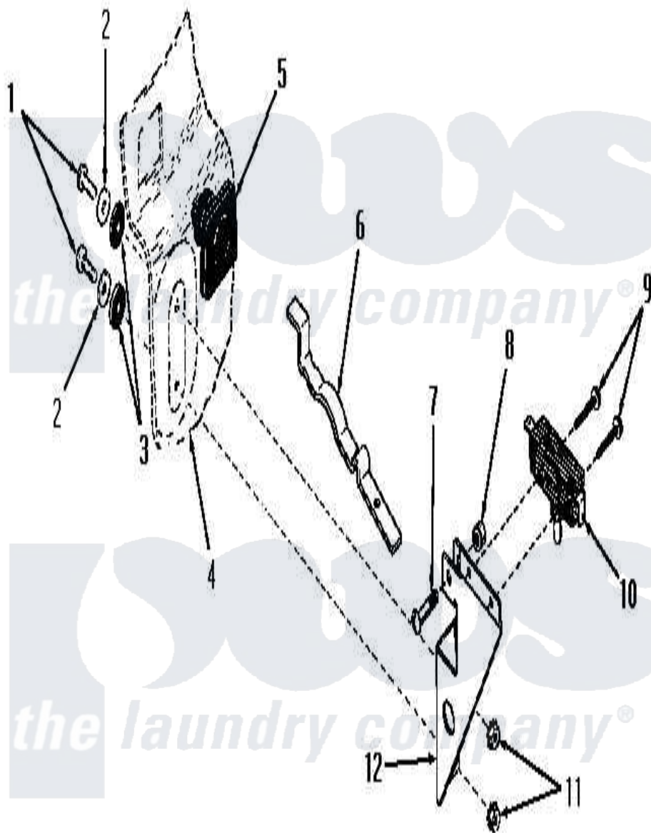
Amana Residential Amana DA6251 Washer Parts Parts Diagram 12 - DOOR SAFETY SWITCH Click on the part number to view part
