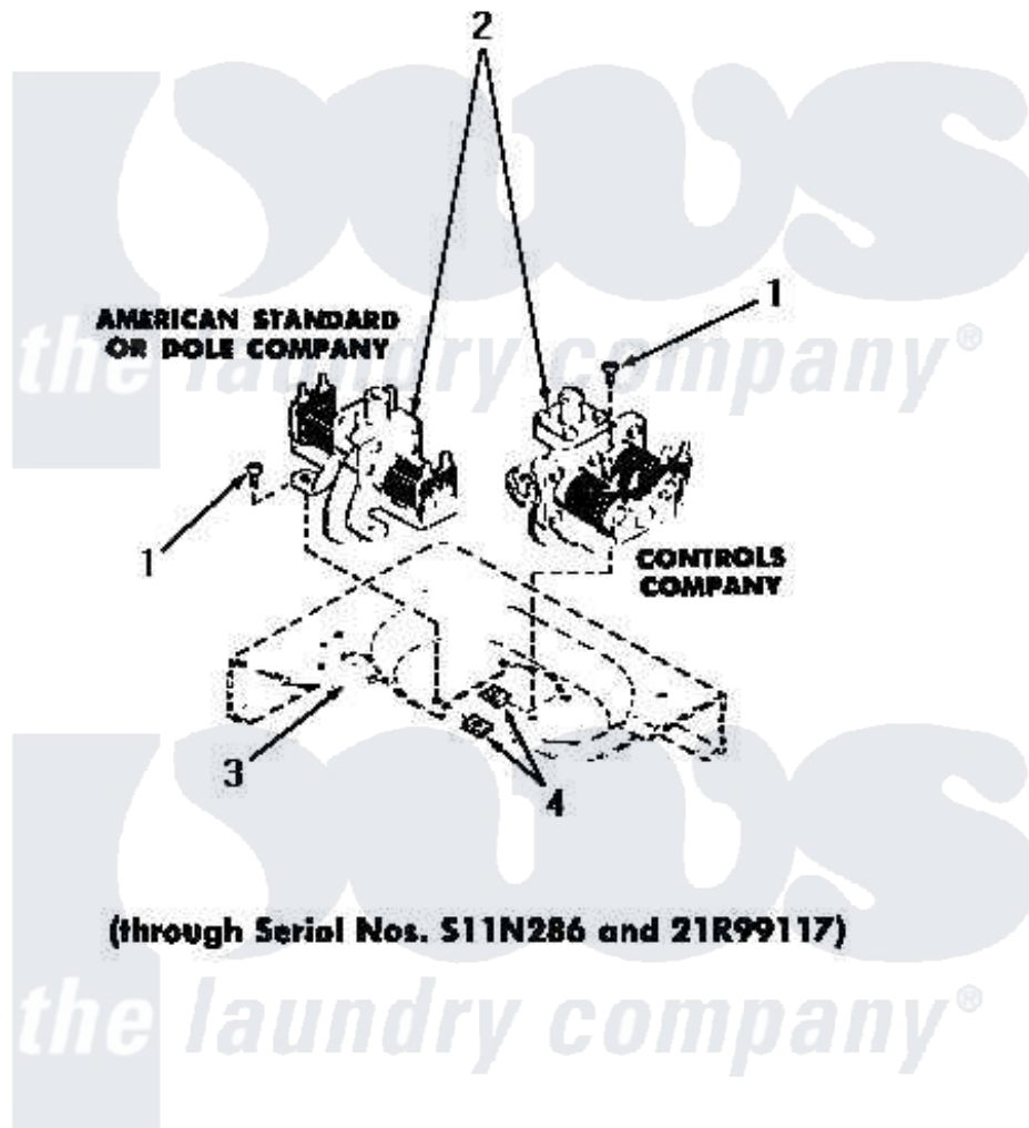
Amana Residential Amana DA9043 Washer Parts Parts Diagram 18 - MIXING VALVES Click on the part number to view part
