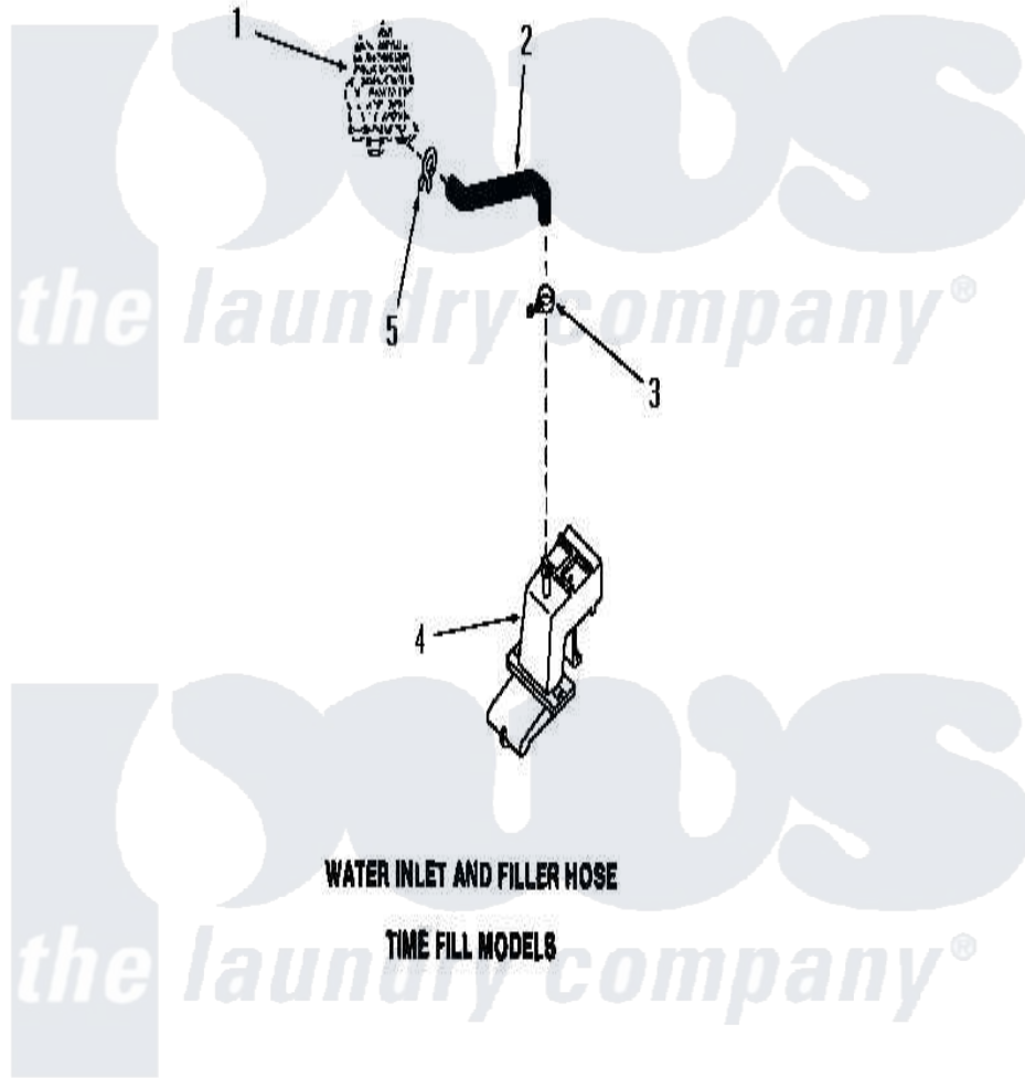
Amana Residential Amana FA3030 Washer Parts Parts Diagram 19 - WATER INLET & FILLER HOSE Click on the part number to view part
