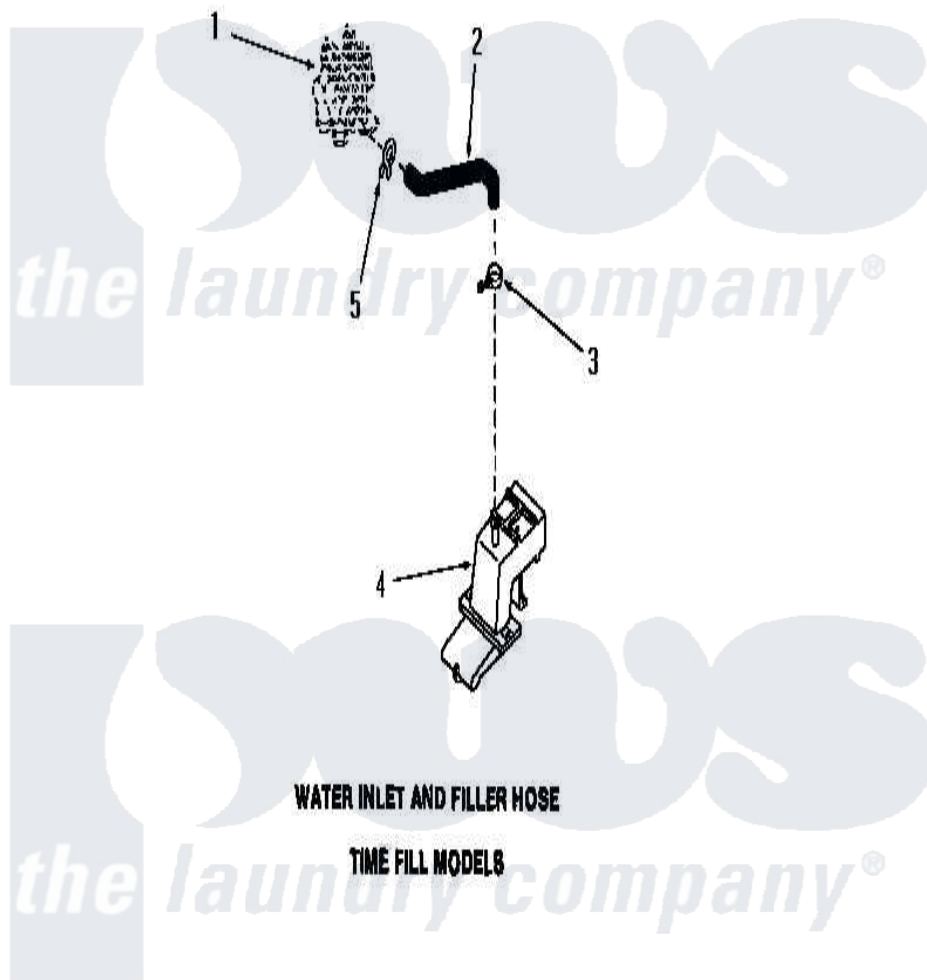
Amana Residential Amana FA3690 Washer Parts Parts Diagram 19 - WATER INLET & FILLER HOSE Click on the part number to view part
