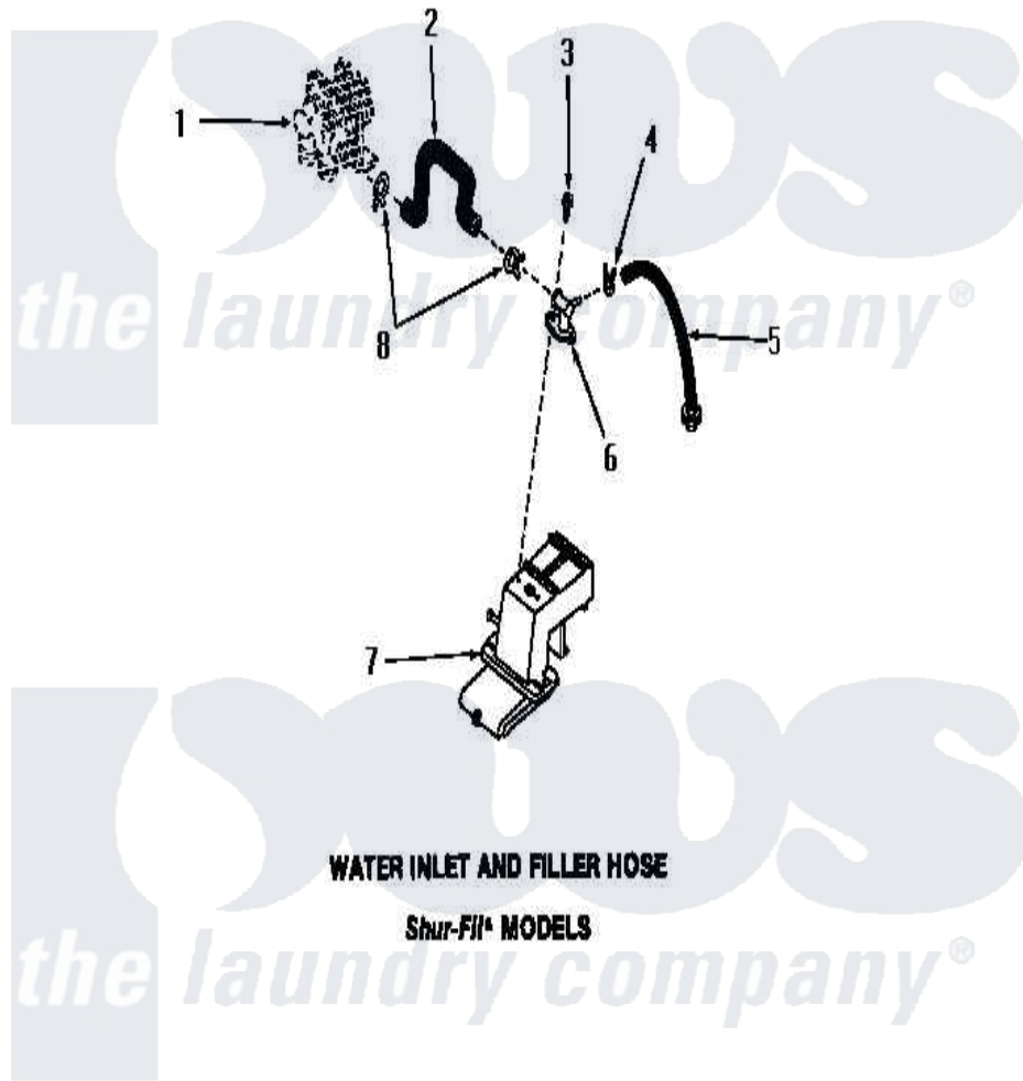
Amana Residential Amana FA4200 Washer Parts Parts Diagram 21 - WATER INLET & FILLER HOSE Click on the part number to view part
