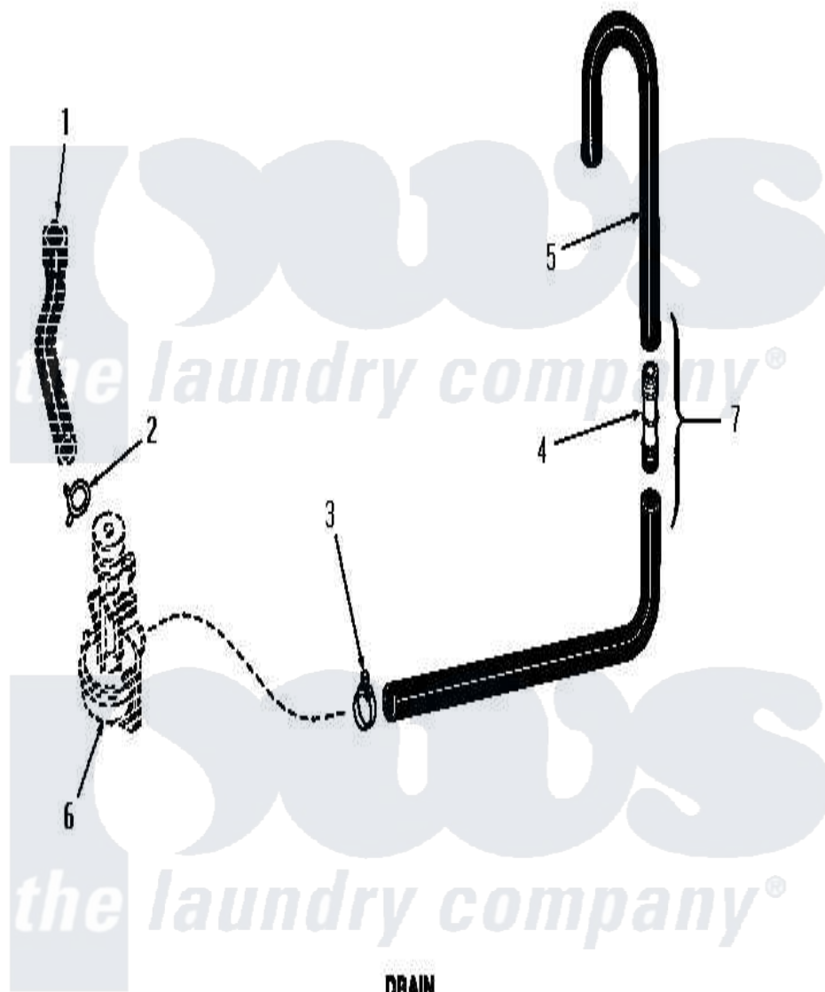
DRAIN
