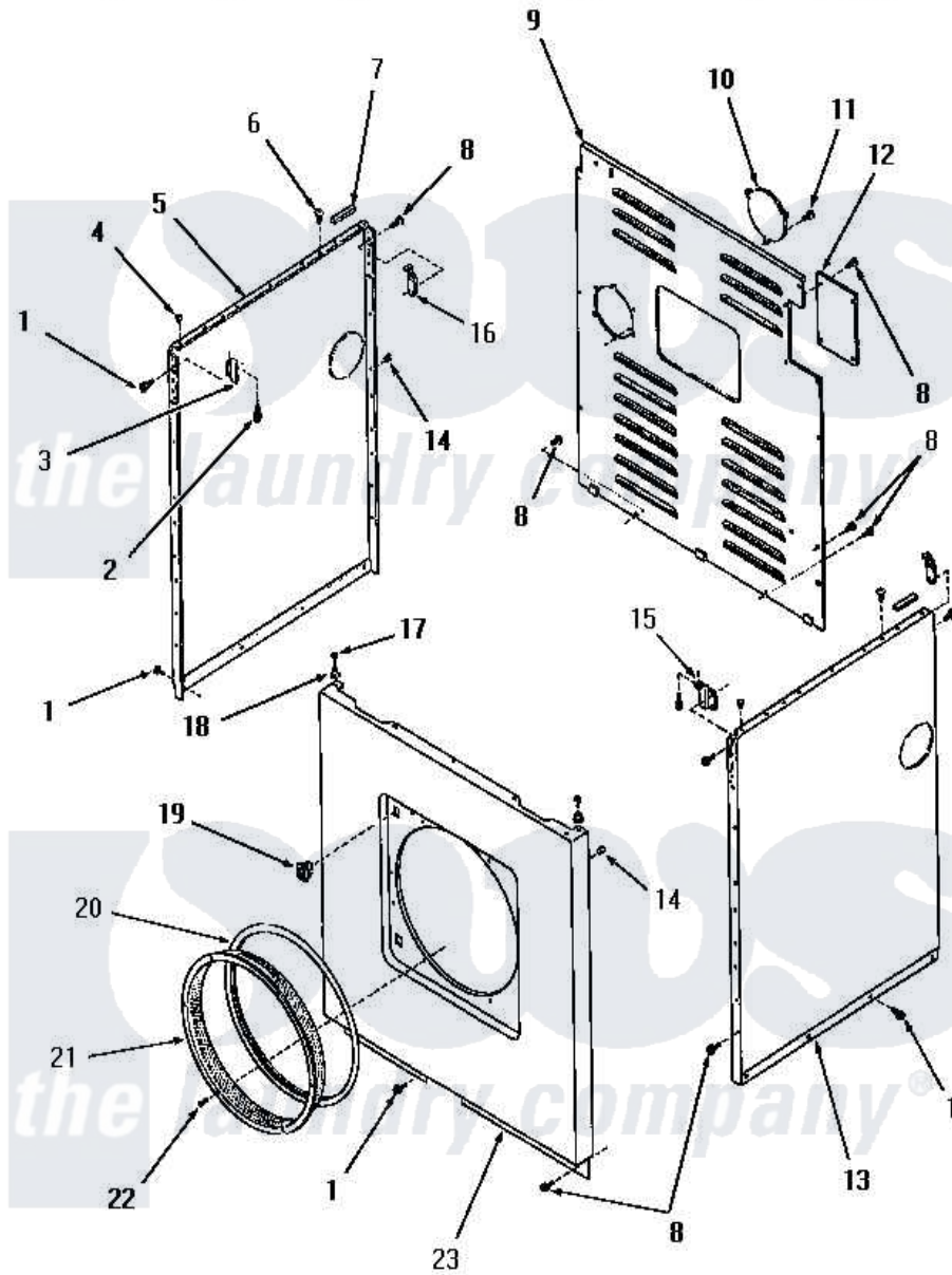
Amana Residential Amana FE6031 Washer Parts Parts Diagram 10 - PANELS Click on the part number to view part
