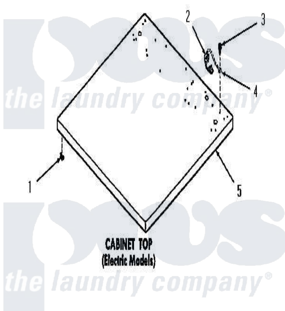
Amana Residential Amana FE6260 Washer Parts Parts Diagram 05 - CABINET TOP Click on the part number to view part
