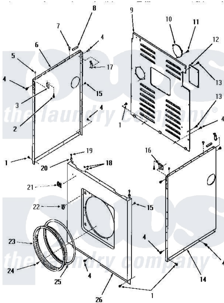
Amana Residential Amana FG6291 Dryer Parts Parts Diagram 12 - PANELS Click on the part number to view part
