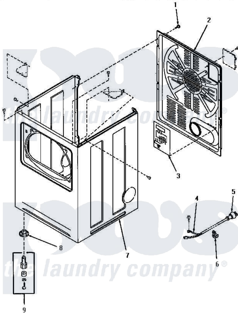
Amana Residential Amana HE1203 Washer Parts Parts Diagram 01 - CABINET ASSY, REAR PANEL AND POWER CORD
