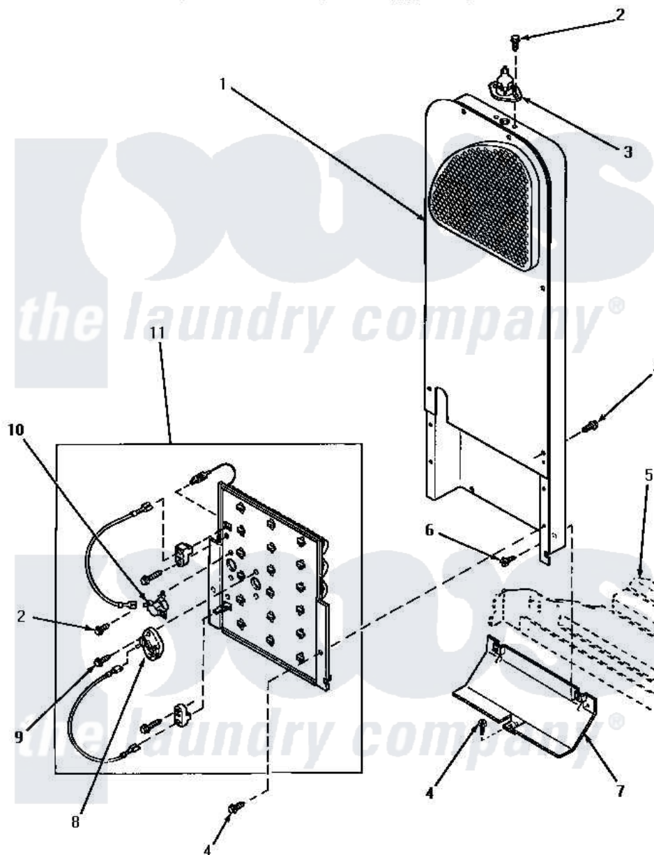
Amana Residential Amana KE5513 Washer Parts Parts Diagram 06 - HEATER BOX Click on the part number to view part
