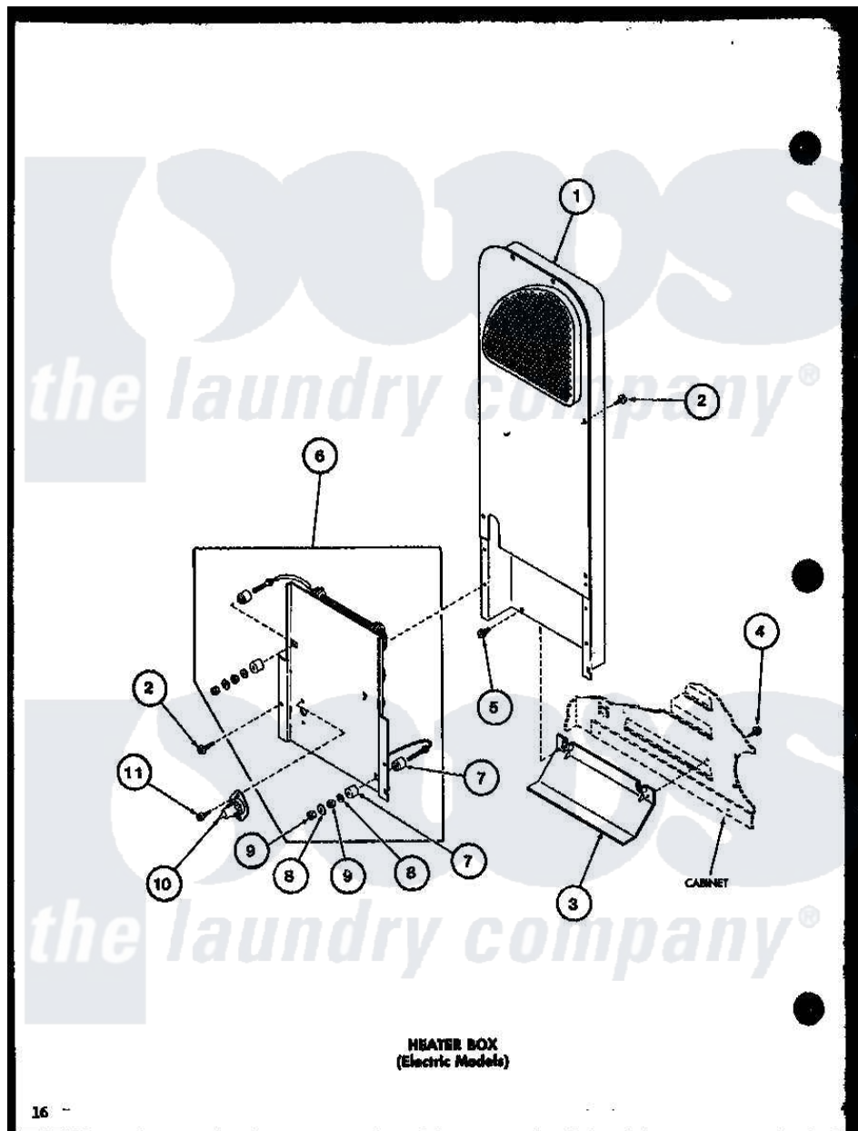
Amana Residential Amana LE1100 (BOM: P7762201W) Dryer Parts Parts Diagram 03 - HEATER BOX (ELECTRIC MODELS)
