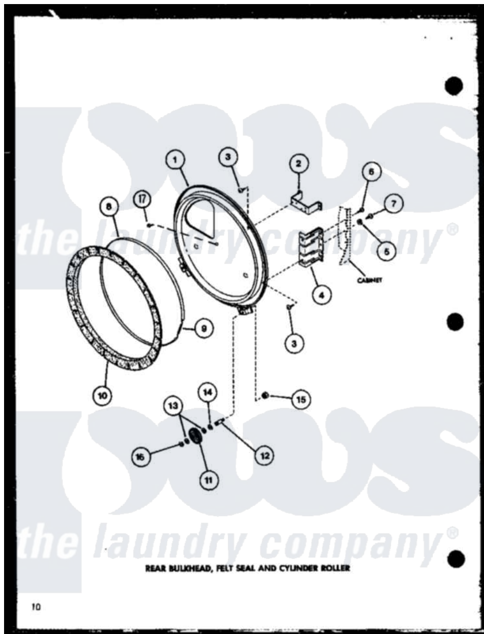
Amana Residential Amana LE1102 (BOM: P7762215W) Washer Parts Parts Diagram 08 - REAR BULKHEAD Click on the part number to view part
