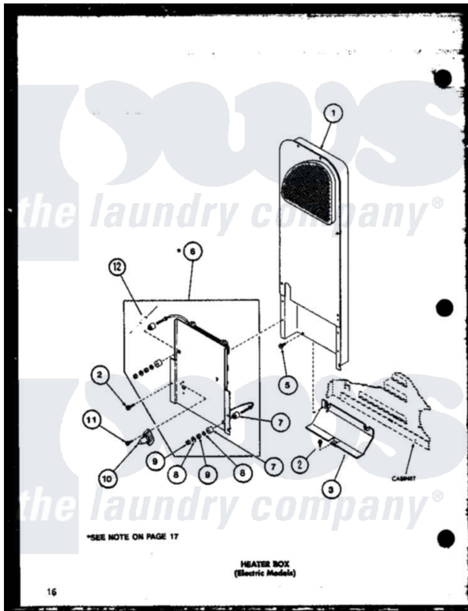
Amana Residential Amana LE2102L (BOM: P1118302W L) Dryer Parts Parts Diagram 03 - HEATER BOX (ELECTRIC MODELS)
