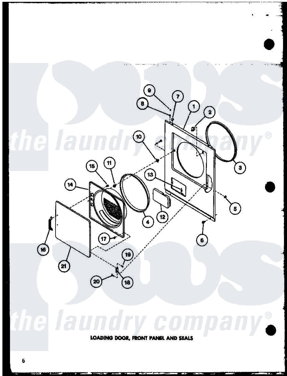
Amana Residential Amana LE2402 (BOM: P7762217W) Washer Parts Parts Diagram 04 - LOADING DOOR Click on the part number to view part
