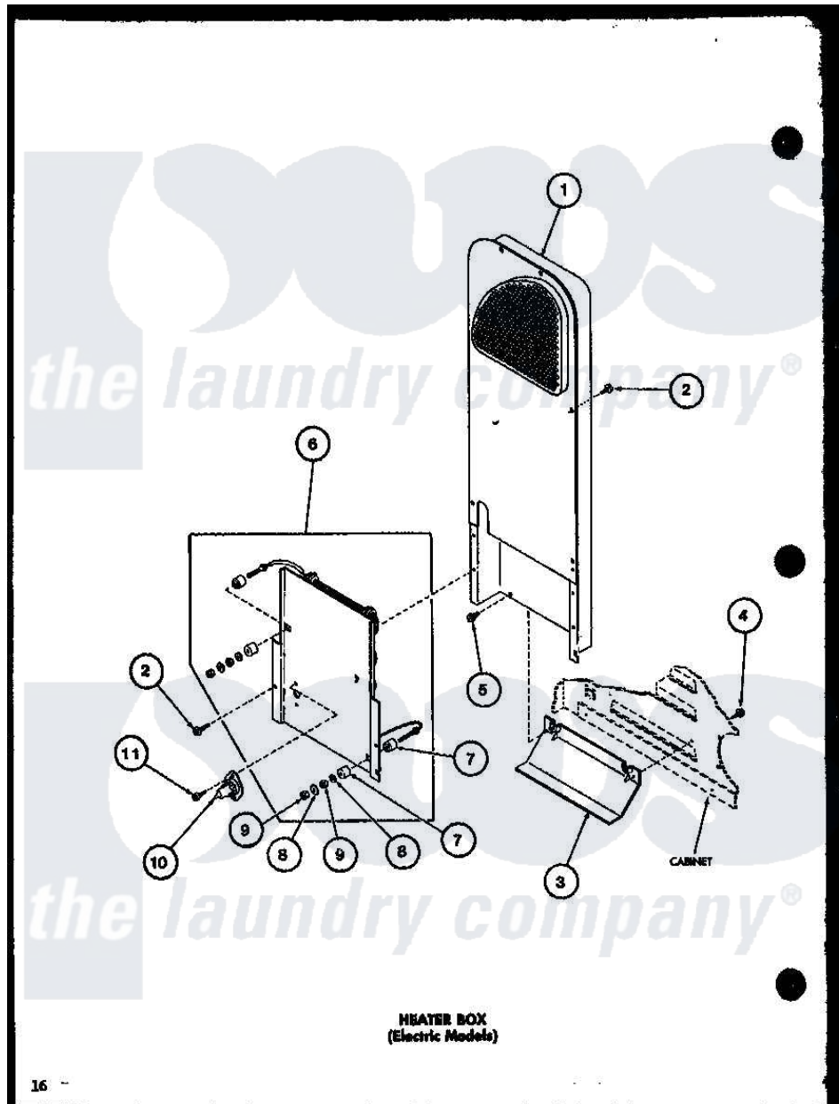
Amana Residential Amana LE2500 (BOM: P7762203W) Dryer Parts Diagram 03 - HEATER BOX (ELECTRIC MODELS)
