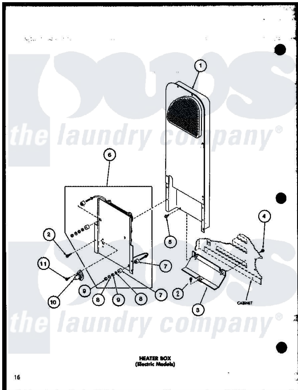
Amana Residential Amana LE2502 (BOM: P7762219W) Washer Parts Parts Diagram 03 - HEATER BOX (ELECTRIC MODELS)
