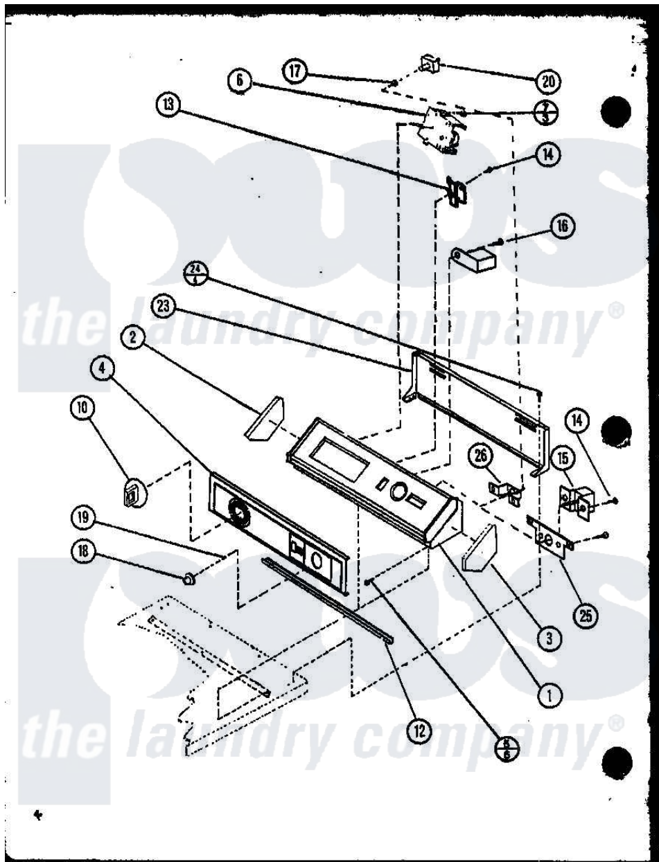
Amana Residential Amana LE2502 (BOM: P7762229W) Dryer Parts Parts Diagram 06 - Page 1
