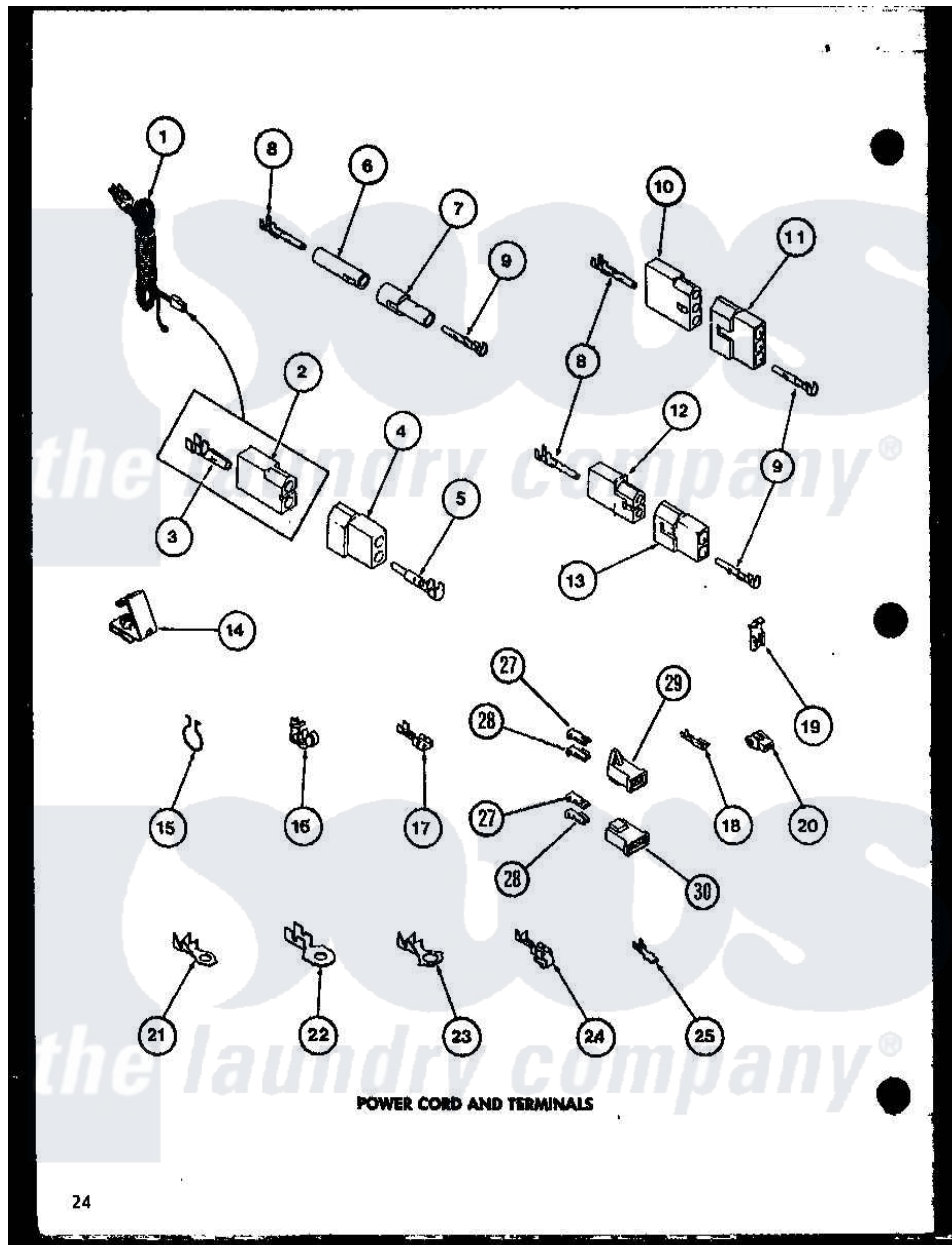
Amana Residential Amana LE2802 (BOM: P7804815W) Washer Parts Parts Diagram 07 - POWER CORD AMD TERMINALS
