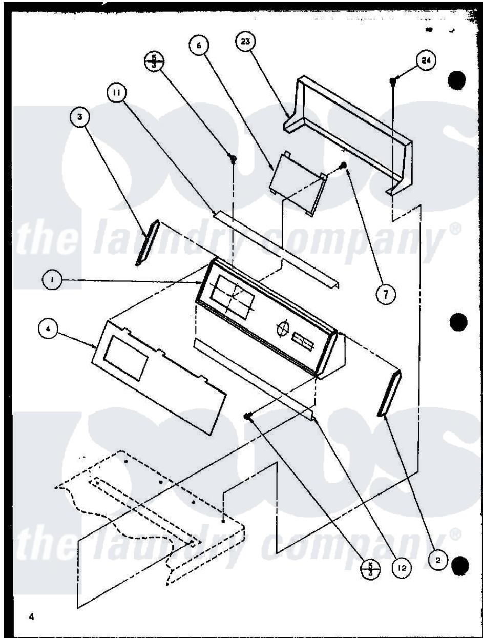
Amana Residential Amana LE2902 (BOM: P7804817W W) Washer Parts Diagram 05 - Page 1 Click on the part number to view part
